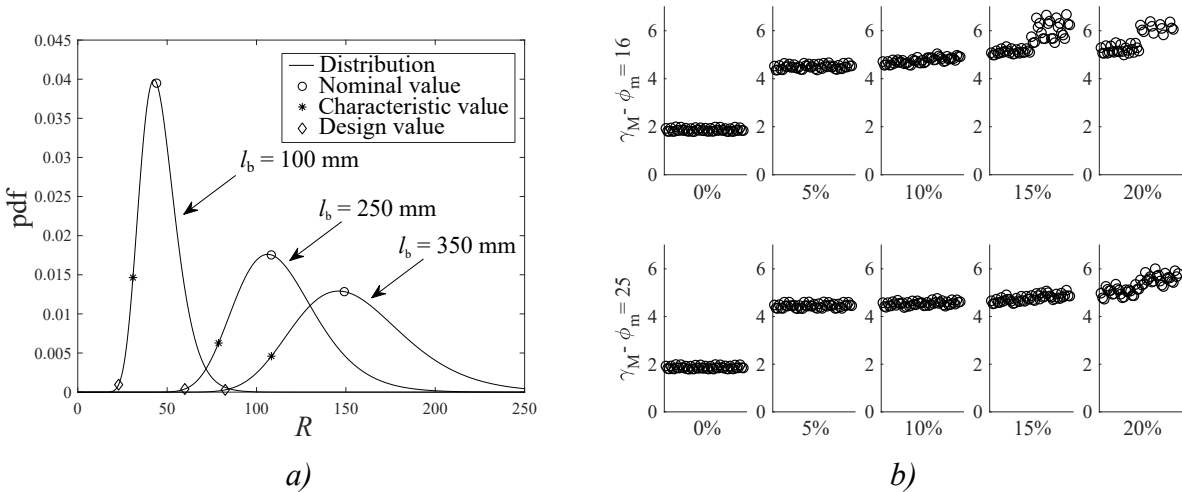
Figure 5.6. a) Probability distributions describing the anchorage capacity for three different embedment lengths for a sample case, plus the nominal, characteristic and design values. b) Comparison of partial factors for two different reinforcement bar diameters for the 480 design cases with stirrups. Adopted from Paper III .
