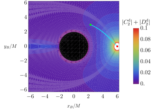
FIG. 2. Direct contributions |C_2^d| + |D_2^d| to the signal strength in the scenario of Fig. 1(b): The detectors are static: Alice is placed at a fixed radial coordinate r_A = 6M , whereas Bob's radial coordinate r_B and angular separation \gamma vary, as labeled by x_B = r_B \cos \gamma and y_B = r_B \sin \gamma . The detector gaps are \Omega_A = 1/M and \Omega_B = 1/(2M) , and Alice couples to the field for her proper time interval 0 \leq \tau_A \leq M . A red dot in Fig. 2b indicates Alice's position, and the plot shows the direct null geodesic emanating from there to the green dot, as one example for Bob's location. Note that the direct contribution is not defined at the exact angular separation \gamma = \pi ; the plot shows a numerical interpolation.
