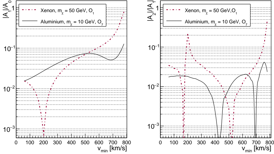
Figure 4.2.6: Hierarchy among the first three higher order harmonics for the two classes of NREFT building blocks . Left: Ratio |A_1|/|A_0| versus v_{min} , for \hat{\mathcal{O}}_1 , class (a), computed for Xe and m_\chi = 50 GeV (dashed-dot purple curve) and for \hat{\mathcal{O}}_7 , class (b), for Al and m_\chi = 10 GeV (solid black curve). Right: Same as left panel, but for the ratio |A_2|/|A_1| .
