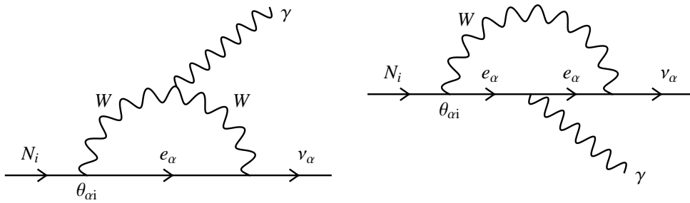
Figure A.2.2: Feynman diagrams of the sterile neutrino radiative decay, allowed by the active-sterile neutrino mixing [105]. N_i and \nu on the diagrams correspond to \nu_s and \nu_a , respectively, in the text.
