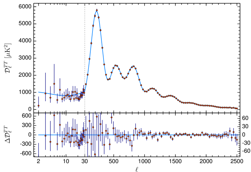
Figure 1.1.1: Multipole moments of the autocorrelation-function of CMB-temperature-fluctuations (Planck Collaboration [55]).
