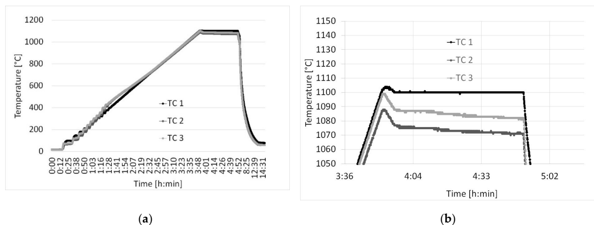
Figure 8. (a) Temperature profile of diffusion bonding experiment with new TC 1 for comparison to old thermocouples. (b) Expanded detail at setpoint temperature of T = 1100\text{ }^{\circ}\text{C} .
