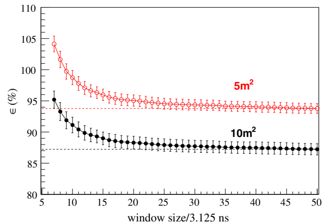
Fig. 5 Efficiency to count individual muons as a function of the time window, for scintillation modules of 10 m 2 (black points and line) and 5 m 2 (red points and line)
