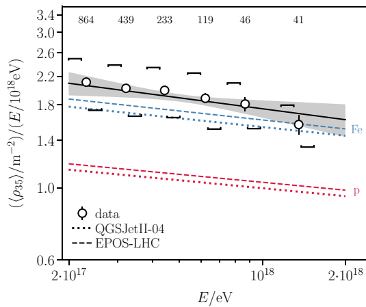
Fig. 11 Energy-normalized muon densities \langle \rho_{35} \rangle / (E / 10^{18} \text{ eV}) as a function of E compared to expectations from simulations using EPOS-LHC (dashed) and QGSJETII-04 (dotted). Error bars denote the statistical uncertainties, while systematic uncertainties are indicated by square brackets
