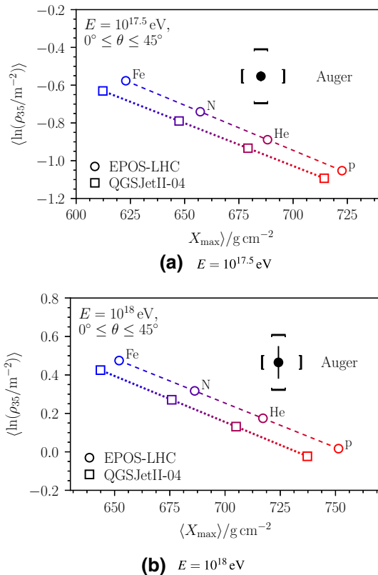
Fig. 12 Mean logarithmic muon density \langle \ln \rho_{35} \rangle as a function of the mean depth of shower maximum \langle X_{\text{max}} \rangle for simulations with primary energies of 10^{17.5} eV (a) and 10^{18} eV (b) compared to Auger Observatory measurements with the FD
