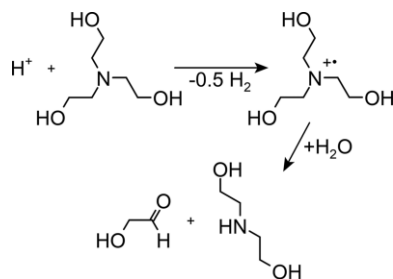
Scheme 1. Reaction pathways of oxidation of TEOA.
