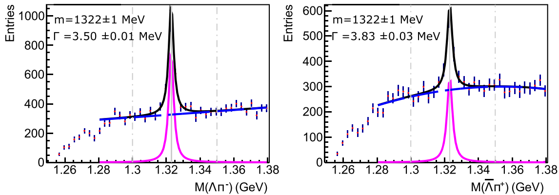
Fig. 2 Left: The \Lambda\pi^- invariant mass spectrum of \Xi^- candidates for rapidity y between -0.25 and 0.25 and transverse momentum p_T from 0.4 to 0.6 \text{GeV}/c . Magenta line represents the fitted Lorentzian function and blue one shows the fitted background, black line represents
