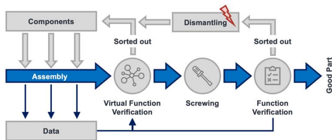
Figure 7: Virtual in-line function verification
