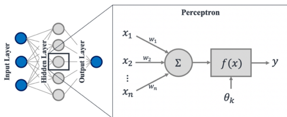
Figure 2: Perceptron and ANN with one hidden layer, cp. [13]
