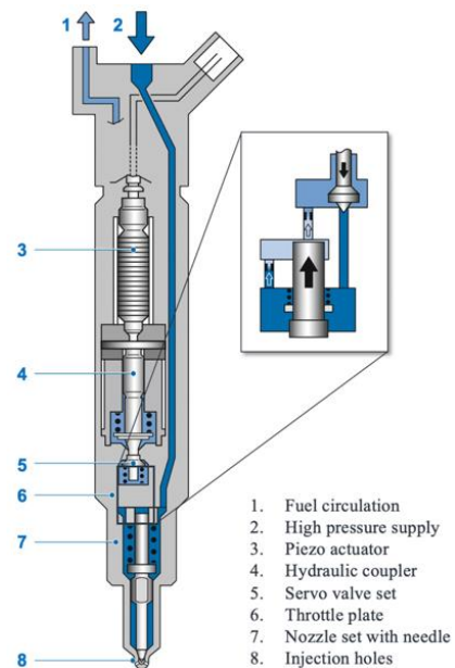
Figure 6: Product principle of a high-pressure injector, cp. [30]
