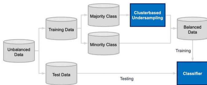
Figure 5: Cluster based under-sampling process [29]
