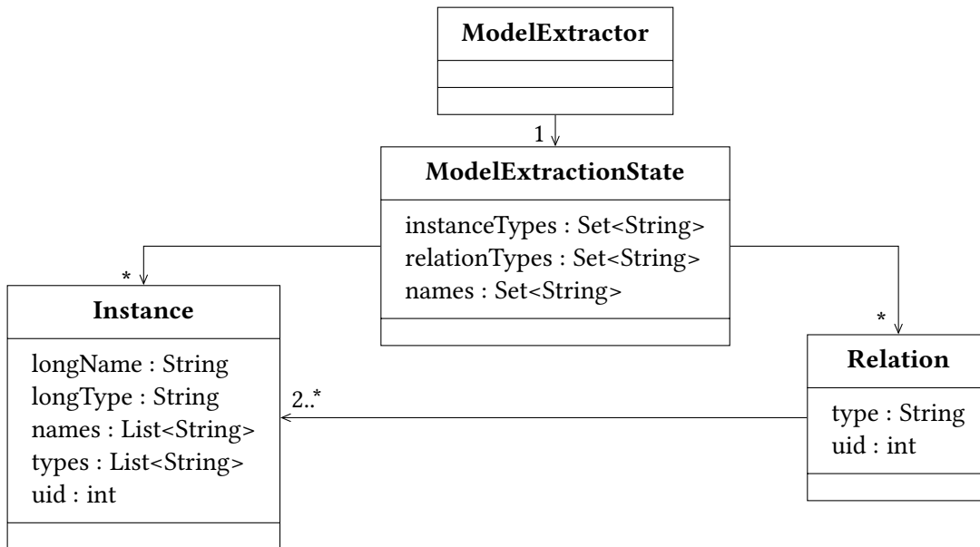
Figure 5.5.: Model Extractor Architecture
