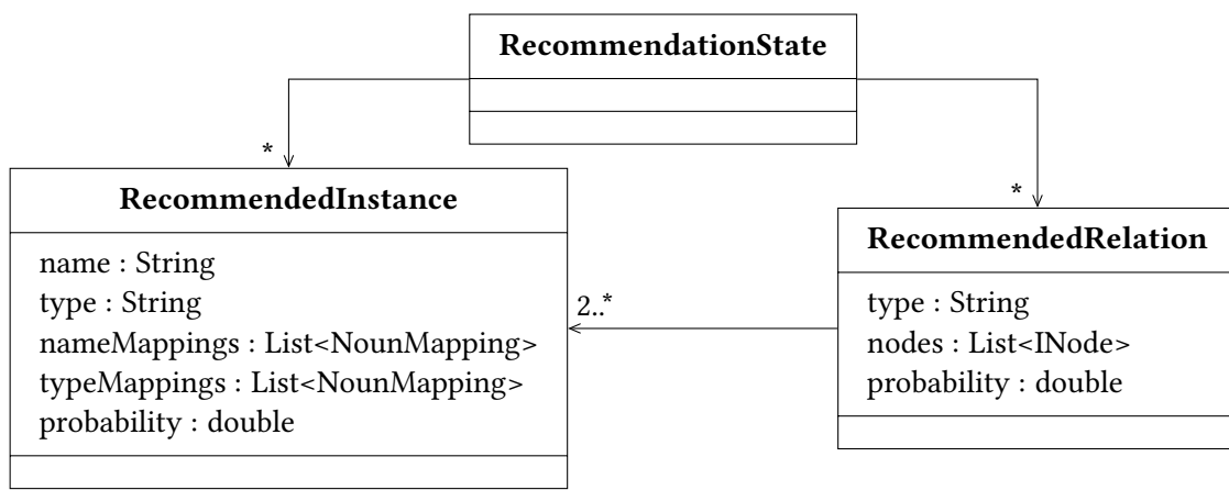
Figure 6.4.: Recommendation Generator
