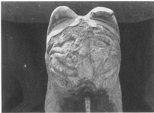
Figure 1 Altered, disaggregated Macael white marble (Patio de los Leones, Alhambra, Granada).
