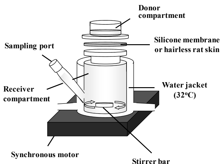
Figure 2. Schematic representation of permeation experiment using silicone membrane and hairless rat skin.
