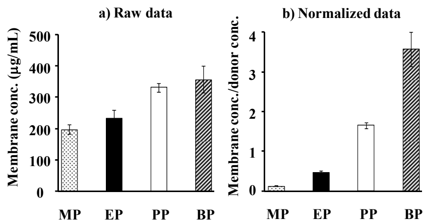
Figure 4. Raw data (a) and normalized data [(silicone membrane concentration)/(donor concentration)] (b) for steady-state silicone membrane concentration of parabens. Each column represents the mean \pm S.E. ( n = 4-8 ).
