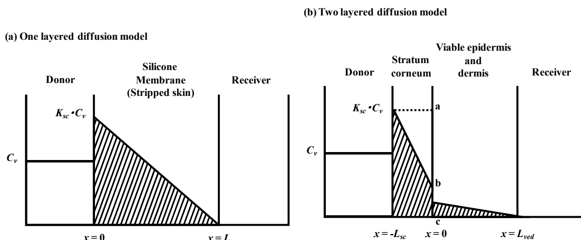
Figure 1. Schematic diagram of concentration-distance profile in one layered (a) and two layered (b) diffusion membrane models in membrane permeation experiments. Membrane thickness is L and L sc + L ved for one- and two-layered diffusion membranes models, respectively. C v is the donor concentration of parabens and K and K sc are partition coefficients to membranes.
