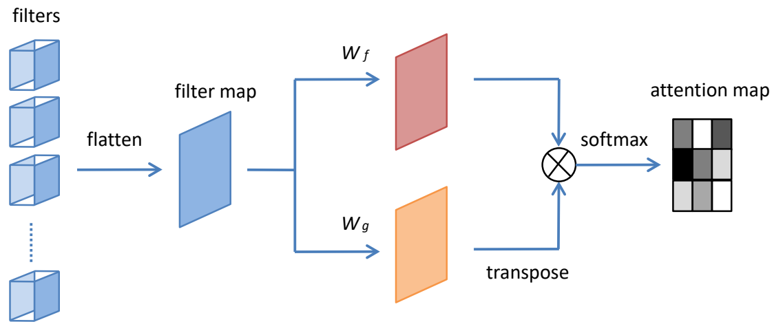
Figure 2. The proposed attention module for PFAM. \otimes denotes the matrix multiplication. The softmax operation is performed on each row.
