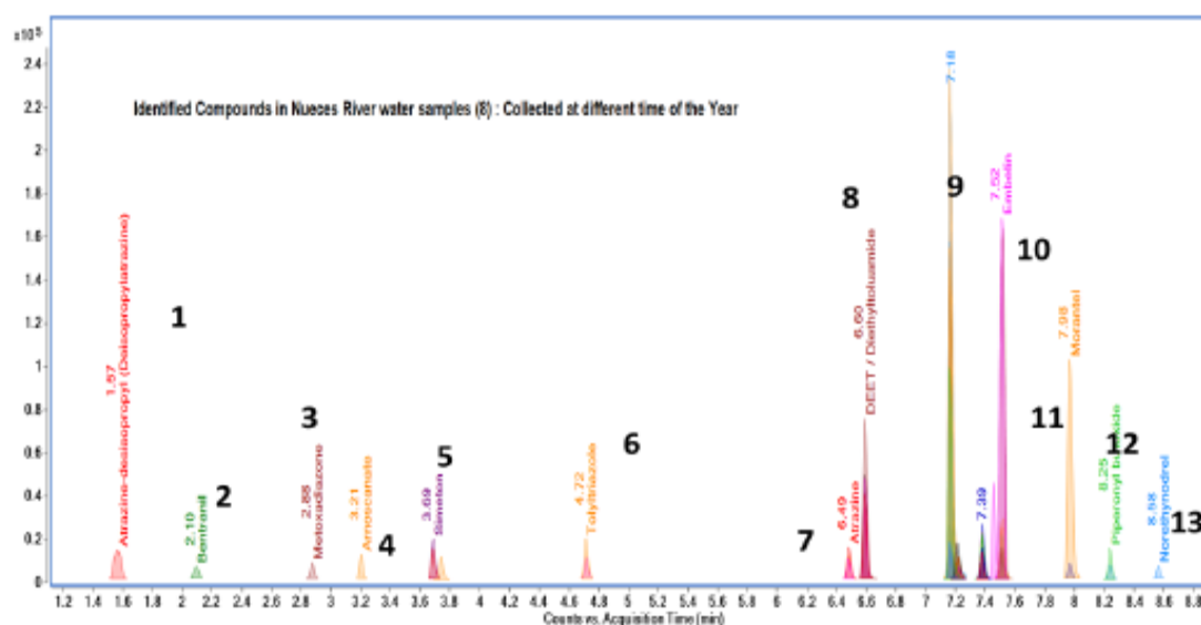
Fig.5. Non-targeted analysis of pesticides and their degradation products in the waters of Nueces river Texas, USA. 1: Deisopropylatrazine; 2: Bentranil; 3: Metoxadiazinone; 4: Arnoscanate; 5: Simeton; 6: Tolyltriazole; 7: Atrazine; 8: DEET/ Diethyltoluamide; 9: Unidentified; 10: Embelin; 11: Morantel; 12: Piperonylbutoxide; 13: Norethynodrel. Complete analytical details are given in experimental section.
