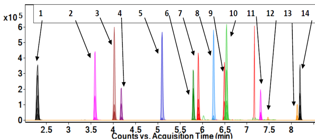
Fig. 1. All ion LC-MS-TOF analysis of fourteen representative pesticides under three fragmentor voltages. Fragments of the parent ion can be seen under the peaks (cf. Fig.2). Complete details are given in experimental section. 1: Aminocarb; 2: Thia-bendazole; 3: Imazapyr; 4: Dimethoate; 5: Metoxuron; 6: Carbofuran; 7: Metosulam; 8: Imazalil; 9: Atrazine; 10: Metazachlor; 11: Malathion; 12: Molinate; 13: Diazinon and 14: Pyraclostrobin.
