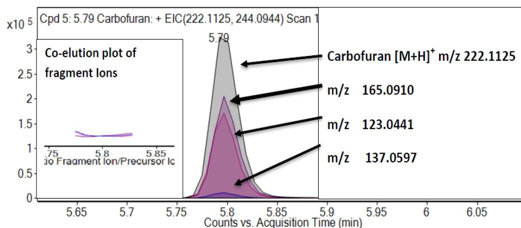
Fig. 2. All ion fragmentation (pseudo MS/MS) of Carbofuran using fragmentor voltage of 150, 200 and 250 V during a single acquisition run. Co-elution plot of fragment ions clearly indicates that all the ions belong to the same parent ion which can be further confirmed by the fragmentation pattern.
