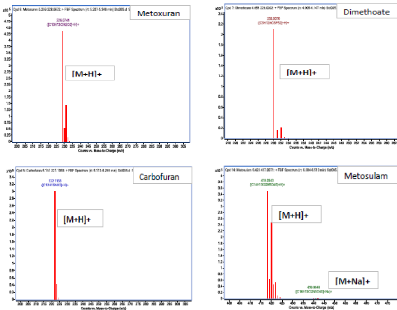
Fig. 3. Mass spectrum of Metoxuran, Dimethoate, Carbofuran and Metosulam obtained using a cocktail of formic acid, trifluoroacetic acid, heptafluorobutyric acid and ammoniumacetate in water-methanol gradient. Near absence of [M+Na]^+ and total absence of [M+K]^+ adducts was observed. Complete LC-MS details under experimental section.
