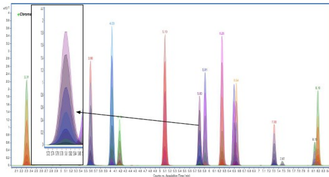
Fig. 4. Chromatograms showing all nine calibration levels of the fourteen representative pesticides. Complete analytical details are given in experimental section. 1: Aminocarb; 2: Thiabendazole; 3: Imazapyr; 4: Dimethoate; 5: Metoxuron; 6: Carbofuran; 7: Metosulam; 8: Imazalil; 9: Atrazine; 10: Metazachlor; 11: Malathion; 12: Molinate; 13: Diazinon and 14: Pyraclostrobin. Inset: Expanded view of Carbofuran calibration levels. All nine levels could be seen with appropriate zooming.
