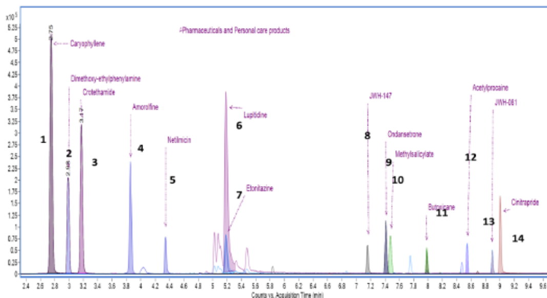
Fig. 7. Non-targeted analysis of Pharmaceuticals and personal care products (PCPs) in the waters of Nueces River, Texas, USA. 1: Caryophyllene; 2: Dimethoxyethylphenylamine; 3: Crothamide; 4: Amorolfine; 5: Netilmicin; 6: Lupitidine; 7: Etonitazine; 8: JWH-147; 9: Ondansetron; 10: Methyl Salicylate; 11: Butoxycaine; 12: Acetylprocaine; 13: JWH-081; 14: Cintrapride. Complete analytical details are given in experimental section.
