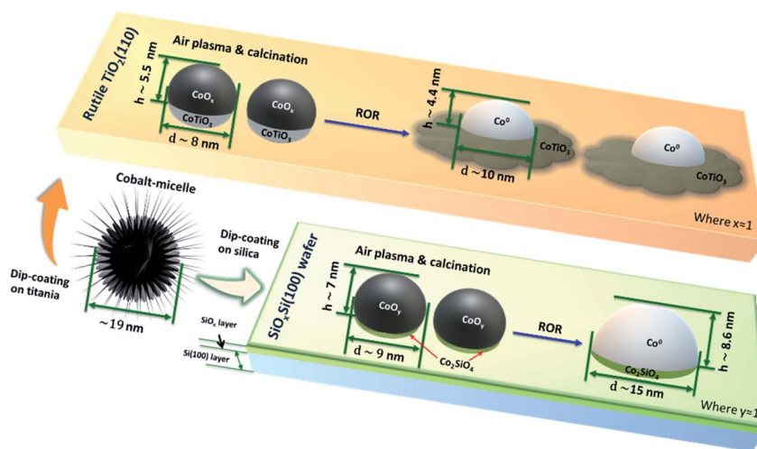
Scheme 1 Schematic of the Co nanoparticles evolution on \text{TiO}_2(110) and \text{SiO}_x\text{Si}(100) substrates after ROR. The spreading of CoNPs onto the surface of \text{TiO}_2 forms a fried-egg shape resulting in strong interaction with the support to form \text{CoTiO}_3 , while CoNPs on \text{SiO}_x\text{Si} tend to move and agglomerate into bigger particles.
