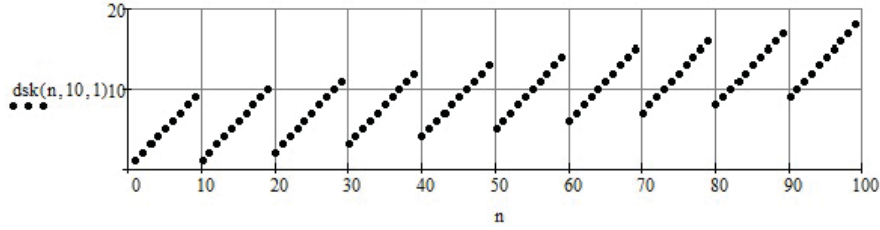
Figure 2.1: The digital sum function
