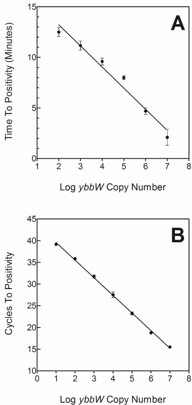
Figure 1. The ybbW target sequence was amplified using either the novel RPA method (A) or an existing qPCR method (B), which targeted the same genetic region in E. coli . The error bars, where visible, represent the standard error of the mean from quadruplicate reactions.
