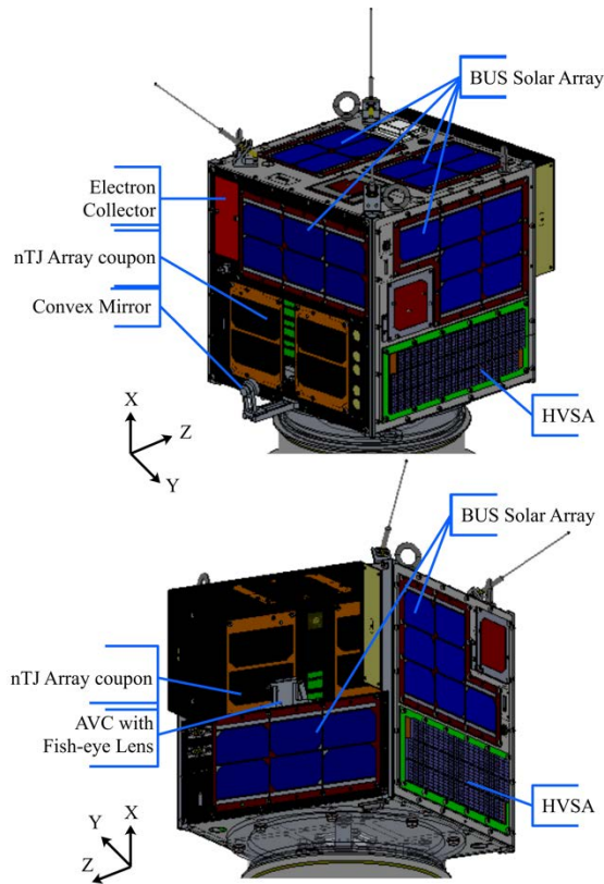
Fig. 2 Exterior of HORYU-IV.
