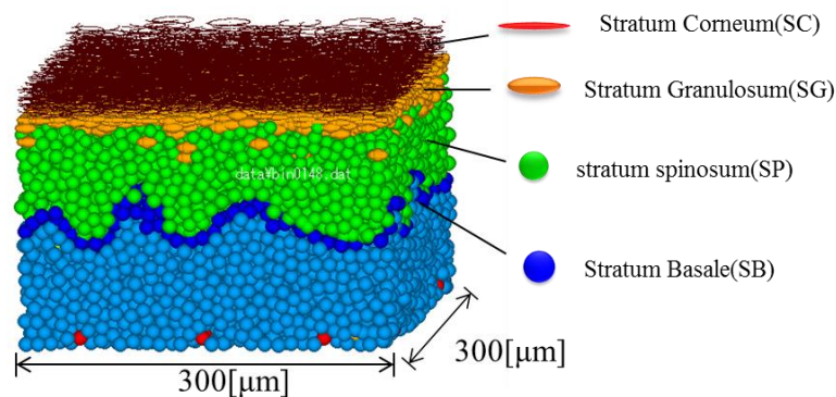
Figure 2. Particle model of keratinization
