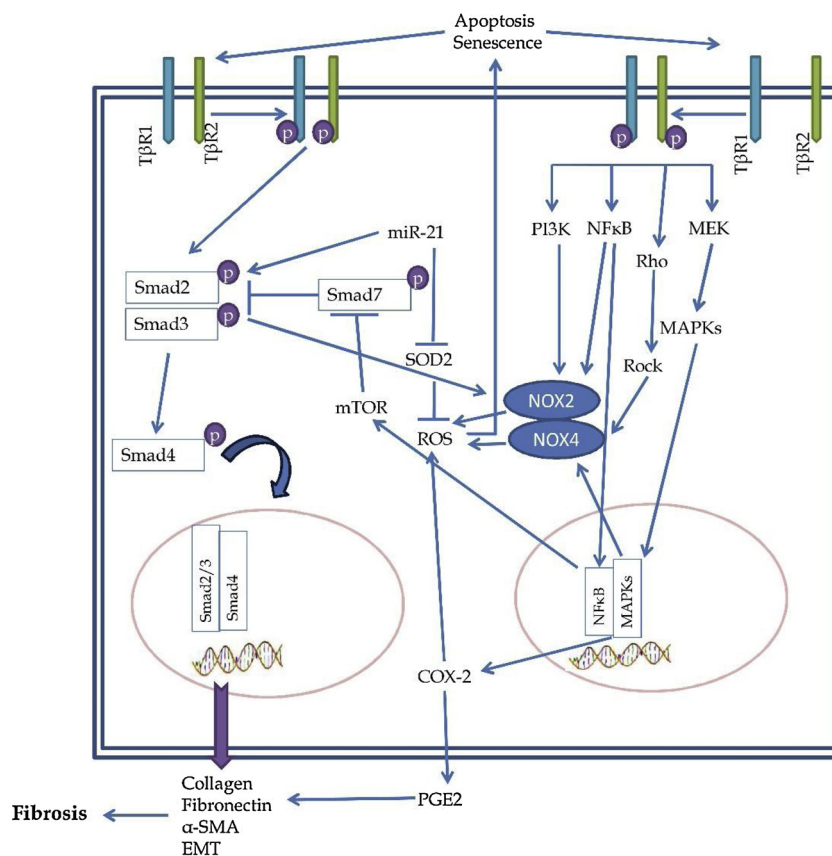
Fig. 3. Mechanisms of TGF- \beta induced fibrosis in irradiated organs. Apoptosis and senescence are the main causes of fibrosis following exposure to high doses of ionizing radiation. Both types of cell death mechanisms are able to trigger fibrosis through stimulation of canonical and non-canonical signaling pathways.
