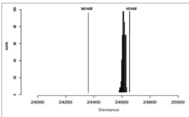
Figure 1: Null model randomization test based on one tree and up to four leaves
