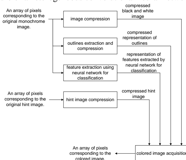
Figure 2. Generalized structure of a neural network solution.
