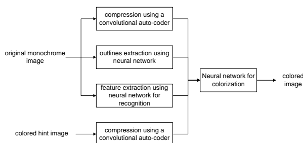
Figure 4. Neural network architecture for colorization.
