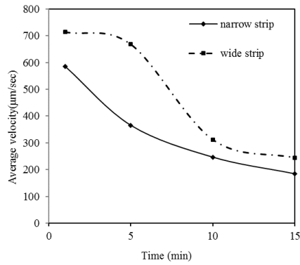
Fig. 2. Effect of width of wicking strip on solution flow
