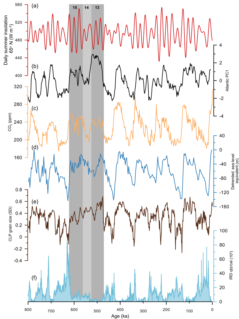
Figure 11. Marine Isotope Stages 15 to 13 and the carbon isotope excursion. (a) Summer insolation at 65°N (red; Laskar et al., 2004). (b) First principal component of Atlantic \delta^{13}\text{C} (black). (c) EPICA Dome C \text{CO}_2 (yellow; EPICA-community-members, 2004; Lüthi et al., 2008). (d) Detrended sea-level equivalent from Shakun et al. (2015) (blue). Derived from \delta^{18}\text{O}_{\text{sw}} calculations. Negative numbers indicate lower sea level and increased ice volume. (e) Chinese Loess Plateau grain size indicating relative Asian summer monsoon strength (brown; Sun and An, 2005). (f) Quartz/calcite ratios from site U1313 in the North Atlantic as a measure of ice-rafted debris (light blue; Naafs et al., 2012). Dark gray bars highlight the interglacials (MIS 15 and MIS 13) between \sim 630 and \sim 470 ka. The light gray bar highlights MIS 14.
