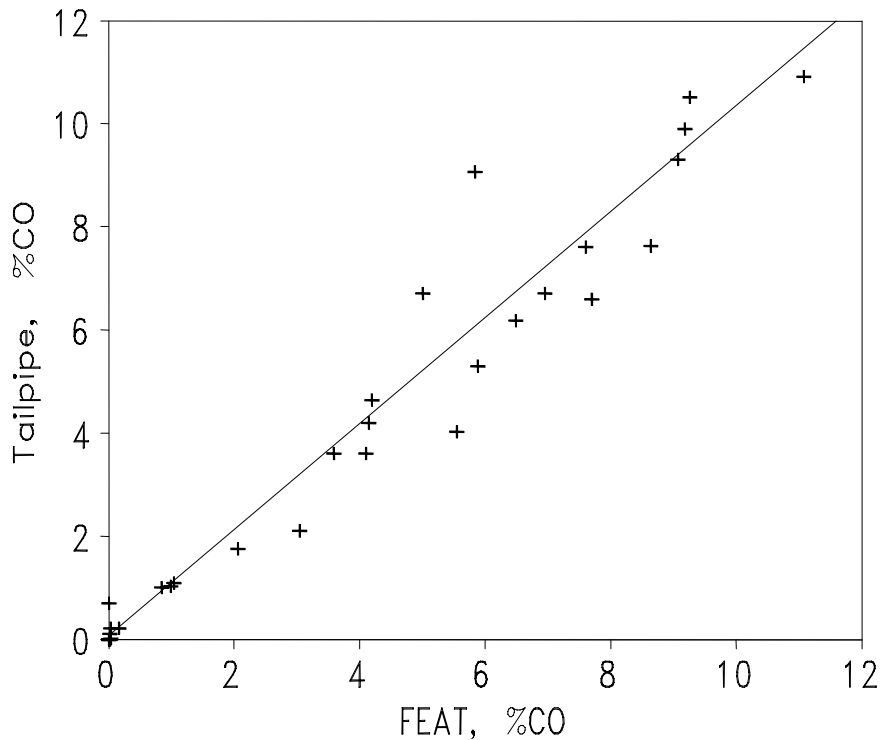
Figure 2. Comparison of tailpipe %CO measured by an on-board analyzer and by remote sensing. Data collected 12/8/89, 12/11/89 and 12/13/89 (n = 34). The equation of the regression line is [\text{Tail pipe \%CO}] = 1.03[\text{FEAT \%CO}] + 0.08 , with r = 0.97 .
