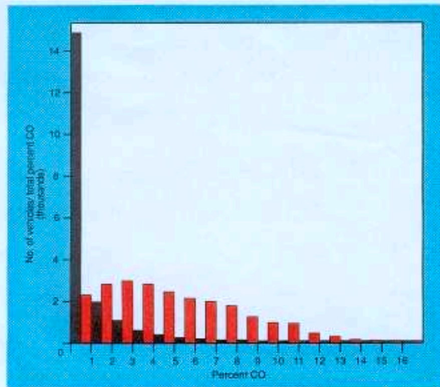
Figure 5. CO emission measurements of operating vehicles made in April 1988 at a local freeway ramp. The black bars represent the number of vehicles measured between adjacent percent CO's (i.e., 0% - 1%, 1% - 2%, etc.). The colored bars represent the total contribution in percent CO for each category.
