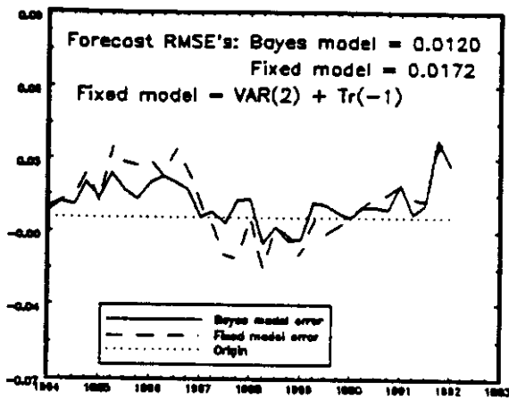
Figure 13: T_Bill -1 : 1959:1 – 1992:1
