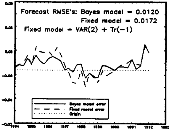
Figure 18: T_Bill -1 : 1959:1 – 1992:1
