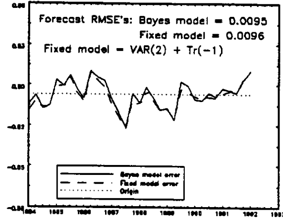
Figure 19: M1: 1959:1–1992:1
