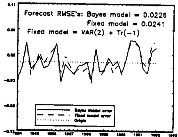
Figure 16: Un: 1959:1–1992:1
