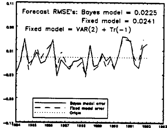
Figure 21: Un: 1959:1–1992:1
