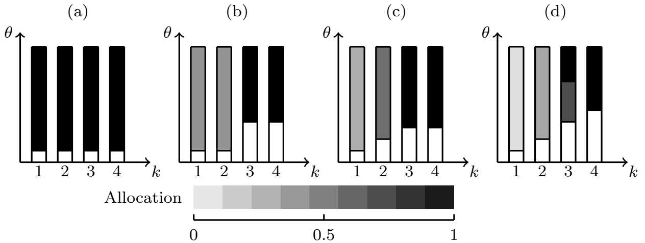
Figure 6: Optimal allocations for K = 4 ; types have exponential distributions with means (2.2, 5.0, 12, 50) (for numerical simplicity, we use truncated versions of these distributions in the interval [0, 60] ). In each panel the vertical axis corresponds to buyers' valuations, and the horizontal axis corresponds to the interim type. Each bar represents the allocation for each type; lighter gray indicates lower probability of allocation, while darker gray indicates a higher probability of allocation. White represents no allocation and black full allocation. From panels (a) to (d), the fractions, \alpha_k , for each type are (0.7, 0.2, 0.05, 0.05) , (0.4, 0.1, 0.4, 0.1) , (0.3, 0.2, 0.4, 0.1) and (0.25, 0.25, 0.1, 0.4) , respectively.
