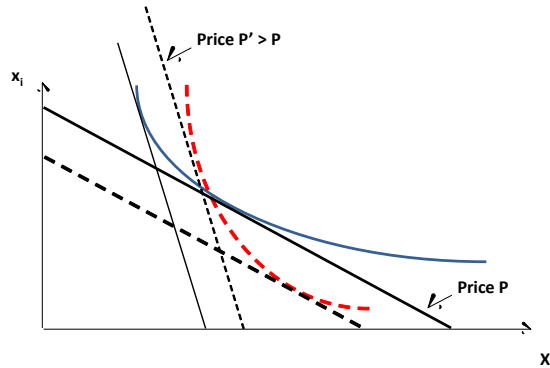
Figure 1: Fig 1: MMWIs for different reference prices
