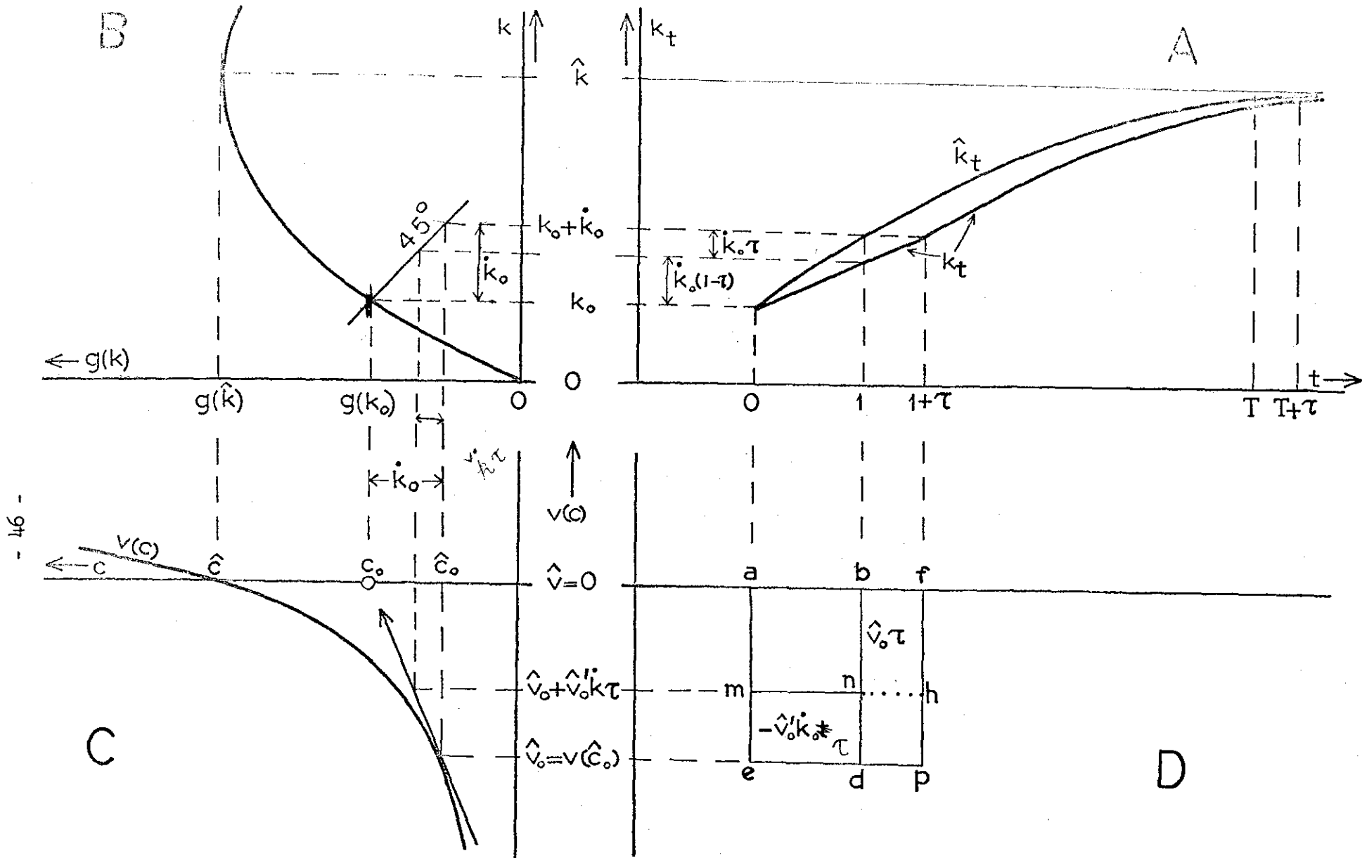
Figure 5 Determination of \dot{k}_0 and \hat{c}_0 .
