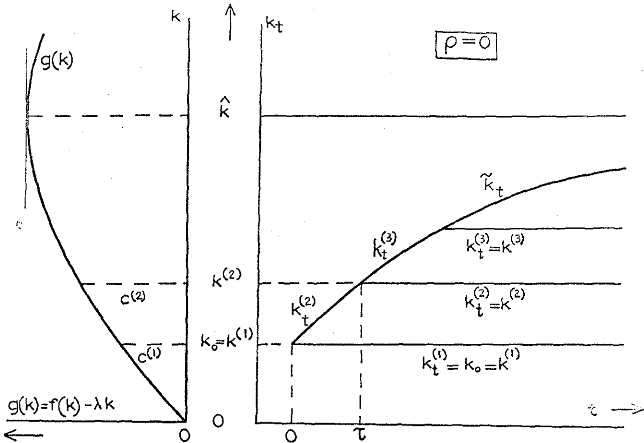
Figure 3 Successively better paths k_t^{(1)} , i = 1, 2, \dots
