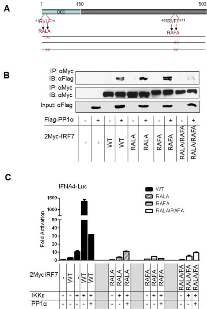
Fig 3. Both PP1-binding motifs on IRF7 are required for its interaction with PP1 and for its activation A. A diagram showing the potential PP1-binding sites on IRF7 and point mutation. B. 293T cells were transfected with Flag-PP1α, 2XMyC-IRF7 or its mutants. Cells were collected for IP with Myc antibody. Immunoblotting was performed with Flag or Myc antibody. C. 293 cells were transfected with 2XMyC-IRF7 or its mutants, IKKε, Flag-PP1α, pGL3/ISRE-Luc, and Renilla. Cells were collected 24 h later for dual luciferase assays. Representative results from three independent transfection experiments are shown.
