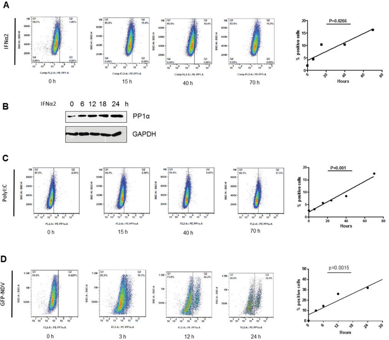
Fig 6. PP1 is induced during antiviral immune responses U937 cells were treated with IFNα2 (A and B), or Poly(I:C) (C), or GFP-NDV (D) at indicated time points. Cells were then fixed and permeabilized before incubation with the mouse anti-PP1α (and then with the F(ab') 2 anti-mouse IgG and analysed by flow cytometry (A, C and D), or subjected to immunoblotting (B), for PP1 expression. Linear regression analysis was performed. *p<0.05 (A), ***p<0.001 (C), **p<0.01 (D). Results are from a single experiment representative of three independent experiments.
