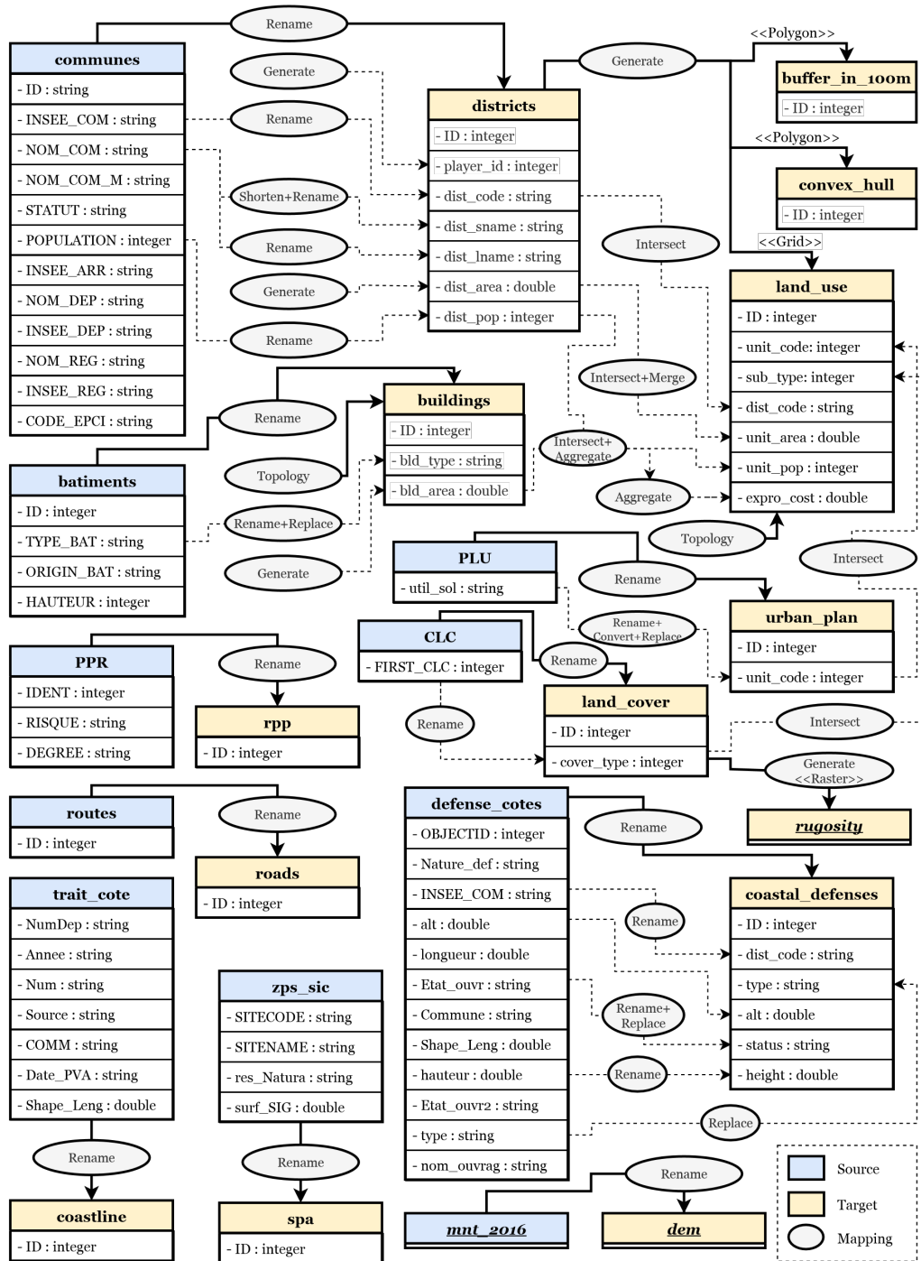
Figure 9. Mapping diagram of LittoSIM data. Blue entities represent the source data. Yellow entities represent the target data. Solid lines (—) link file mapping patterns. Dashed lines (---) link attribute mapping patterns.
