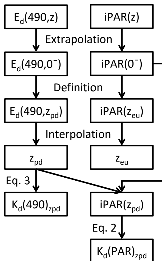
Figure 2. Flow chart of BGC-Argo radiometry data processing. Note that all derived K_d values are layer-averaged ones (the layer from sea surface to depth z , thus, z as the subscript in the symbols, e.g., K_d(490)_z ), rather than K_d at a specific depth. The same procedure could be used to derive the layer-averaged attenuation coefficient to any depth of interest.
