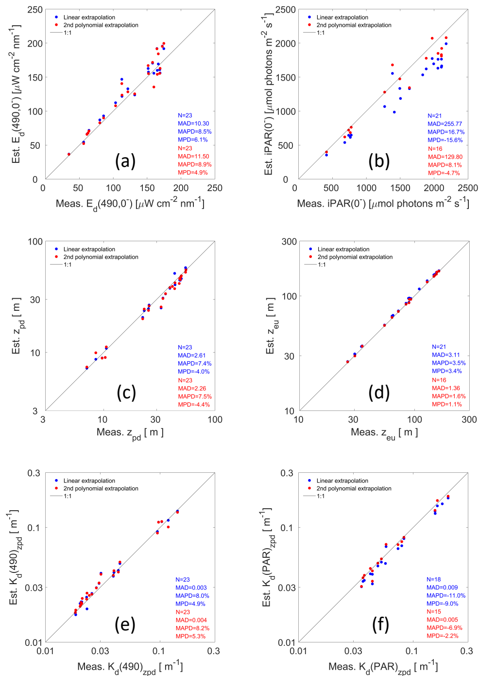
Figure A1. Evaluation of BGC-Argo data processing methods suggested here using the BIOSOPE data. Scatter plot of Measured and Estimated values, of E_d(490,0^-) (a) i\text{PAR}(0^-) , (b) z_{pd} , (c) z_{eu} , (d) K_d(490)_{zpd} , (e) and K_d(\text{PAR})_{zpd} , (f) respectively. “Measured (meas.)” means determination of E_d(490,0^-) and i\text{PAR}(0^-) based on measured radiometry above sea surface; “Estimated (Est.)” means determination of E_d(490,0^-) and i\text{PAR}(0^-) is based on a linear (blue) or second-degree polynomial extrapolation (red) within the upper 10 m of the ocean. The black solid lines represent the 1:1 lines.
