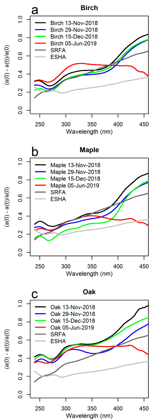
Figure 1. Change in absorption following borohydride treatment for (a) birch leachates, (b) maple leachates, and (c) oak leachates. All leaf litter leachates, excluding maple 15 December 2018 displayed higher loss of UV absorption following treatment. Additionally, the litter from June 2019 all displayed decreased response to borohydride from 400–500 nm in relation to the autumn leachates and reference standards.
