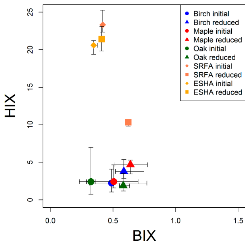
Figure 4. Mean, biological index (BIX), and humification index (HIX) for leaf litter leachates. Leaf litter and planktonic chromophoric dissolved organic matter (CDOM) exhibit low HIX, but slightly different BIX (BIX characterizes shape of emission at 310 nm excitation. HIX characterizes shape of emission at 255 excitation). Suwannee River Fulvic Acid (SRFA) decrease in HIX following treatment is not observed in other samples, including Elliot Soil Humic Acid (ESHA). Error bars represent the range of values for all four time points for each species.
