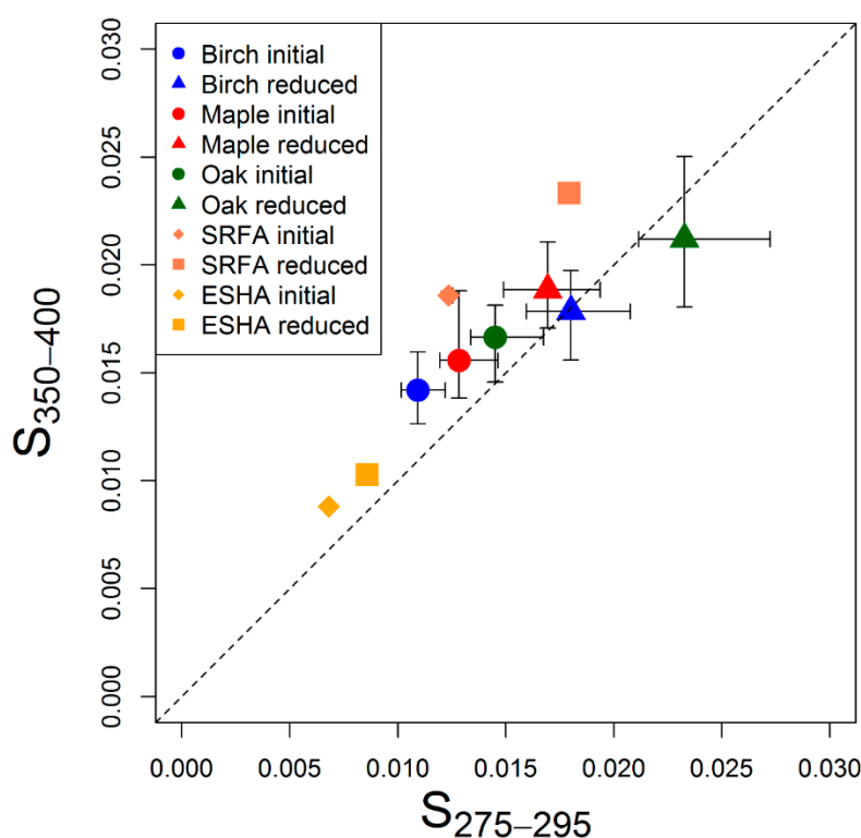
Figure 2. Mean absorption indices, S_{275-295} and S_{350-400} , for leaf litter leachates. Borohydride treatment (reduced) causes increases in both metrics for all samples. Both spectral slopes do not appear to distinguish leaf leachates from HA and FA standards. Error bars indicate range of values for all four time points of each species. Dashed line indicates a spectral ratio of 1.
