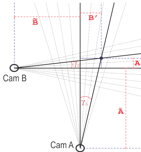
Figure A1. An illustration of the basic coordinate system used to find the area for each pixel, drawn for a simplified 8 pixel \times 8 pixel geometry. Following the notational conventions established in the appendix, the dotted exemplar vertex corresponds to m = 3 and n = 2 .
