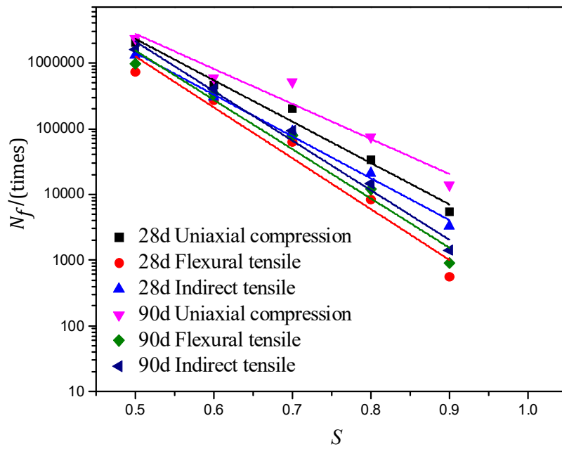
Figure 7. Fitting curve for the fatigue equation for a cement content of 4% under different stress states.
