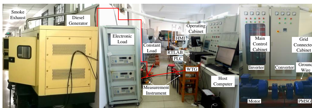
Figure 9. Experimental platform.
