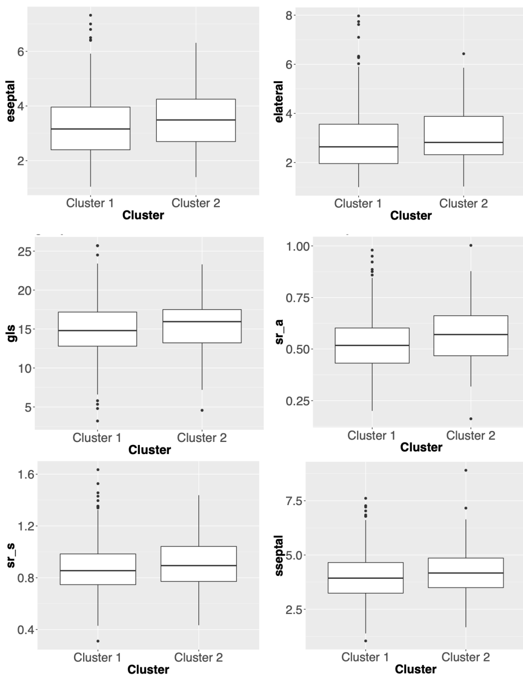
Figure 3. Box plots of phenotypic/outcome variables whose distributions are significantly different between two clusters in Caucasian cohort. The p -values for eseptal, elateral, gls, sr_a, sr_s and sseptal are 0.0135, 0.0465, 0.0246, 0.0151, 0.0774, 0.0879 respectively.
