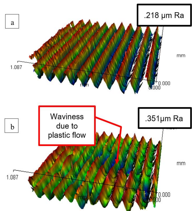
Fig. 6. Laser interferometer-generated surfaces showing the roughness increase due to sideflow and stability issues cutting with larger hones for the same nose radius. a) 1.6mm nose radius, 0.1mm feed, 5\mu\text{m} hone. b) 1.6mm nose radius, 0.1mm feed, 50\mu\text{m} hone.
