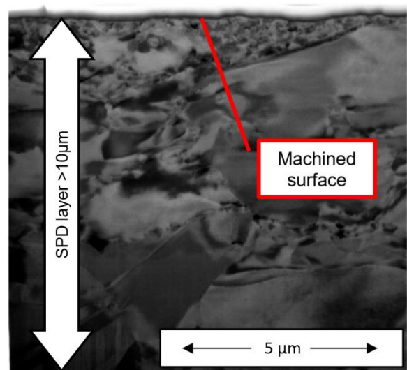
Fig. 8. FIB micrograph of near-surface microstructure of sample machined with 50 \mu\text{m} hone, 0.4mm tool nose radius and 0.1mm feed. The SPD layer continues well into the subsurface. FIB microscopy, 10000x.
