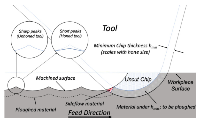
Fig. 3. Geometrical model of a turning process clarifying the influence of ploughing effects on roughness at higher kinematic roughness values. Note that h_{min} is meant to denote minimum chip thickness.
