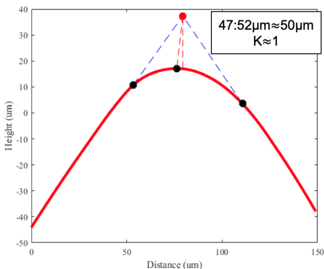
Fig. 2. Example of characterization method employed to analyze the cutting edge micro-geometry of cutting tools used in the experiment.
