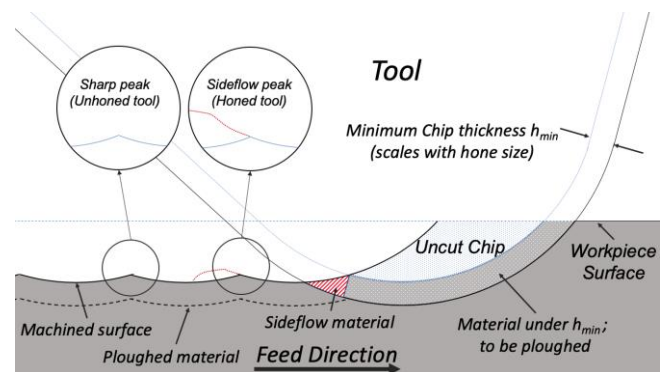
Fig. 4. Geometrical model of a turning process depicting ploughing effects on roughness at lower kinematic roughness values. Note that h_{min} is meant to denote minimum chip thickness.
