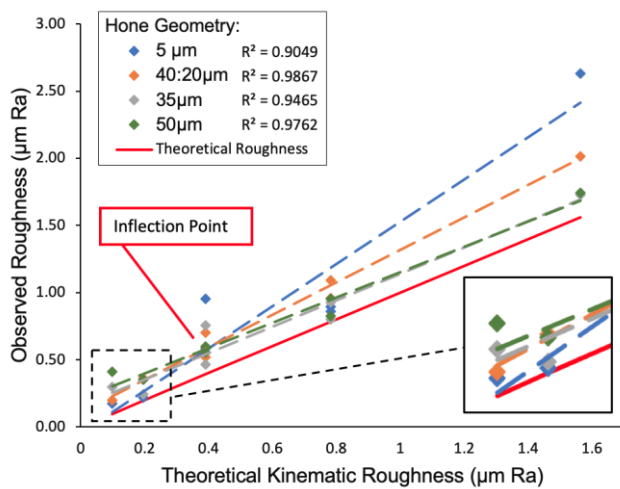
Fig. 5. Graph showing the roughness trends for each hone.
