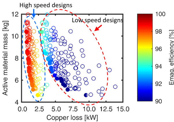
Figure 4. Optimization results for the high speed WAVED motor together with designs obtained by scaling for the higher torque and lower speed at the same power ratings.
