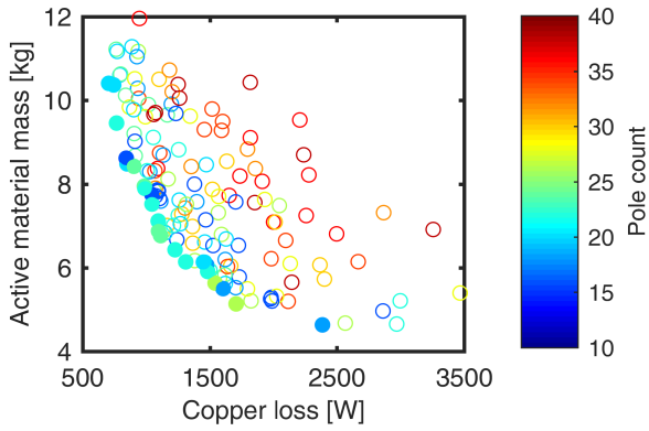
Figure 3. Optimization results for the high speed WAVED motor. The Pareto front designs are shown with filled markers and the color map is for the number of poles.
