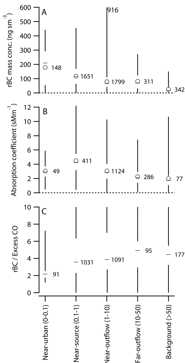
Fig. 11. Whisker plots showing the mean (circles), median (horizontal dash), minimum, maximum, 25th and 75th percentiles (vertical lines) classified by air mass type for (a) refractory black carbon (rBC) mass, (b) light absorption coefficient at 550 nm, and (c) ratio of rBC to excess carbon monoxide mixing ratios ( \text{ng s m}^{-3}/\text{ppbv} ). Air masses are defined using ratios of \text{O}_3/\text{NO}_x (listed with air mass label) following Morgan et al. (2010a). The number of individual data points in each bin are given to the right of the data. Maximum rBC/CO ratios are truncated to 10 and only median values are shown due to bias from high ratios associated with variability in the rBC/CO ratios.
