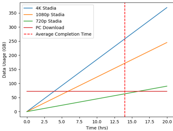
Figure 1: How game play time affects data volume for Metro Exodus on Stadia.
