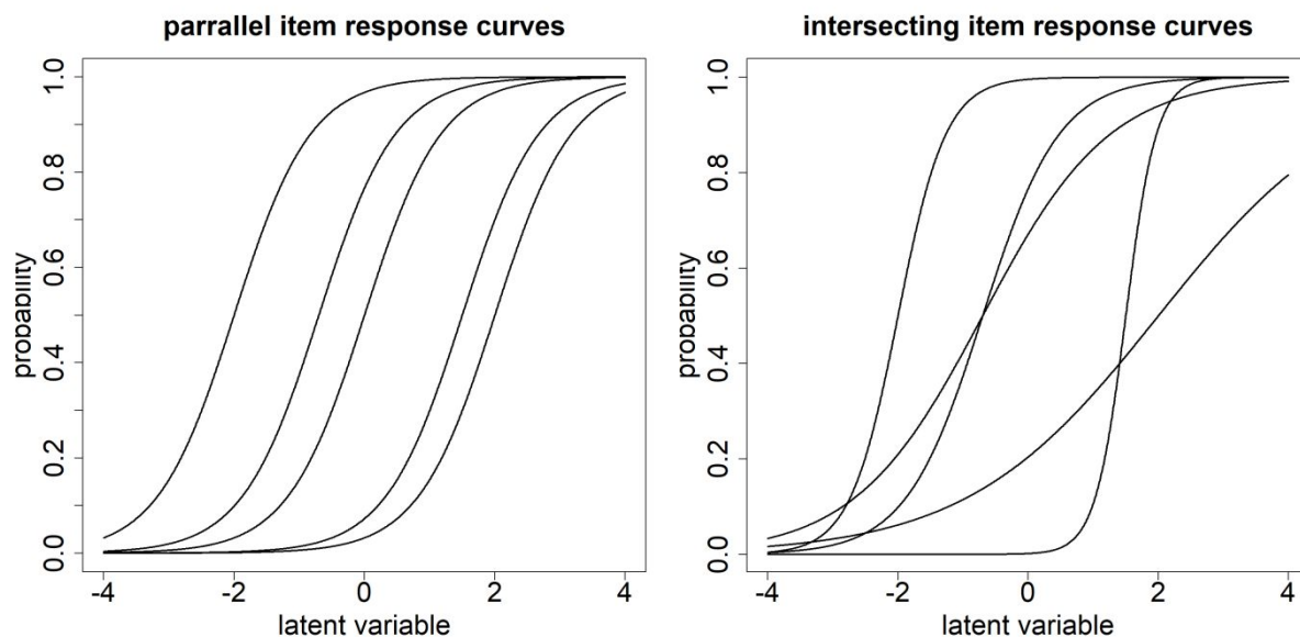
Figure A1: Examples of item response curves for parallel (left) and non-parallel (right) for binary scored items
