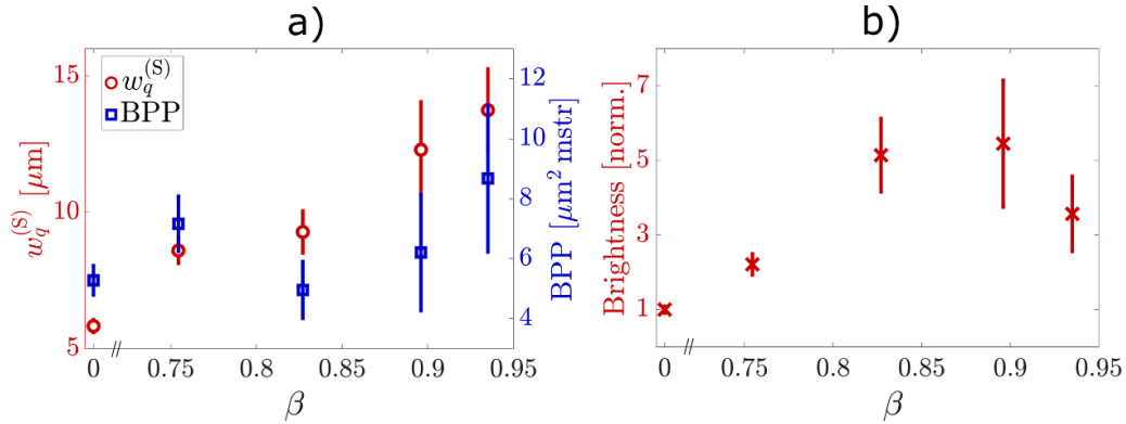
Figure 5. (a) Measured w_q^{(s)} (red open circles) and BPP (blue open squares) as a function of \beta . (b) Measured harmonic brightness as a function of \beta .
