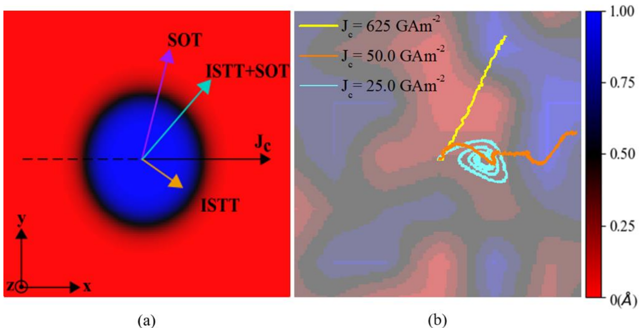
FIG. 1. (a) A snapshot of a 400 nm diameter Néel skyrmion, showing the z magnetization component. The magenta, orange and cyan arrows represent the direction in which the SOT, ISTT and the combination of these two torques in the spin transport solver act on the skyrmion when a current is applied, respectively. The black arrow indicates the conventional current direction, J_c . (b) Skyrmion motion in a bilayer system displaying pinned, creep and flow regimes in cyan, orange, and yellow, respectively. The contoured effect outlines the disordered pattern on the surface of the sample with depth displayed by the heatmap. All paths were obtained using a damping constant \alpha = 0.03 and disorder variation period of 60 nm.
