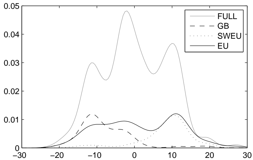
Figure 8. Kernel estimates of the PDF of jet latitude, as in Figure 1, but for days exhibiting blocking over different locations (GB: Greenland Blocking, 53^{\circ}\text{N} , 50^{\circ}\text{W} ); SWEU: South-west Europe, 41^{\circ}\text{N} , 15^{\circ}\text{W} ); EU: Europe, 53^{\circ}\text{N} , 15^{\circ}\text{E} ). The PDF of the full dataset is shown in grey and the other PDFs have been scaled by the number of days in each set.
