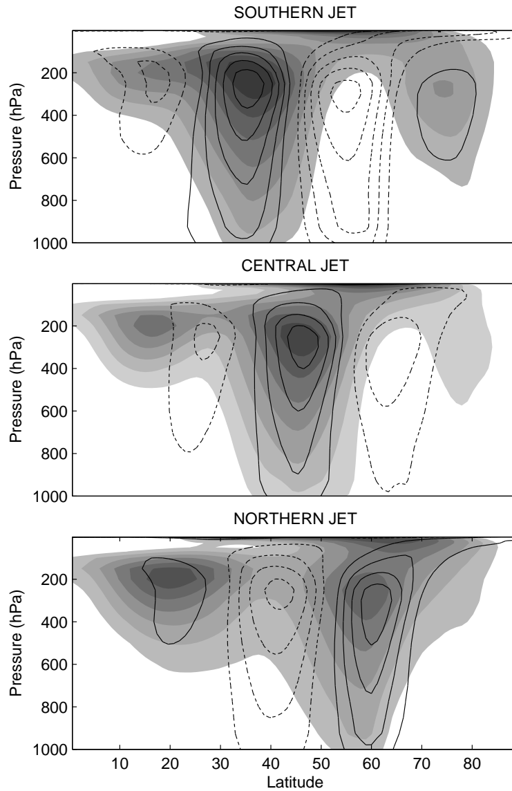
Figure 5. Composites of the zonal wind averaged over 0–60°W for the three jet stream locations. Shading shows the full field contoured every 5 \text{ms}^{-1} , with the lowest contour drawn at 5 \text{ms}^{-1} . Contour lines show anomalies from the DJF climatology at 3 \text{ms}^{-1} intervals, with negative contours dashed and the zero contour omitted.
