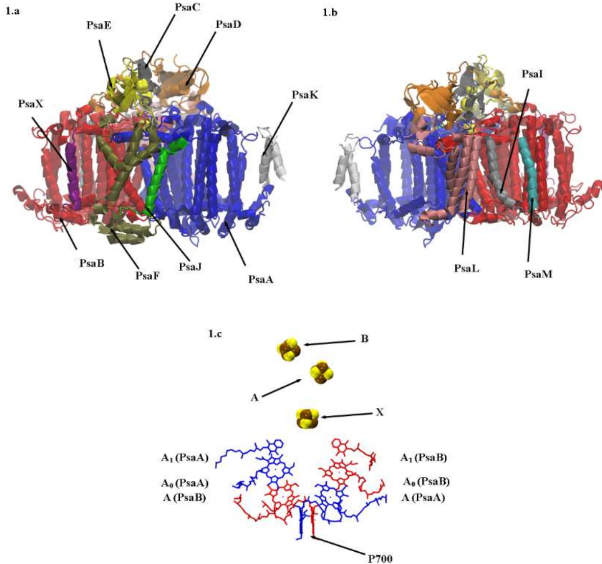
Figure 1. [PDB code 1JB0 12 ] : 12 protein-subunits in the polypeptide structure of Cyanobacterial PS I monomer viewed perpendicular of the plane of the thylakoid membranes. 1.a: Front view and 1.b: Back view while 1.c: Shows the electron transfer chains ETCs in PS I, where P700 is primary electron donor (Chl a dimer), primary electron acceptors A /A 0 (Chl a molecules), secondary electron acceptor A 1 ( Phylloquinone molecule PQN), tertiary electron acceptor X (F X ) and terminal electron acceptor A (F A ) and B (F B ) 8
