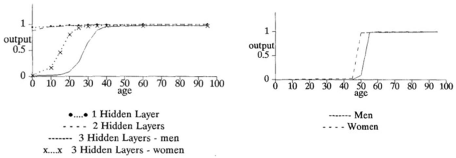
Fig. 12 Neural networks and open texture (Bench-Capon 1993)
