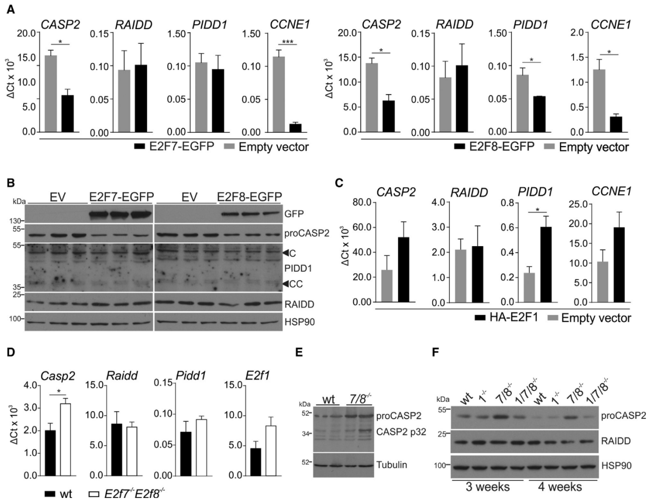
Figure 7. An E2F1/E2F7/E2F8 Autoregulatory Loop Controls PIDD1 and CASP2 Expression Levels
