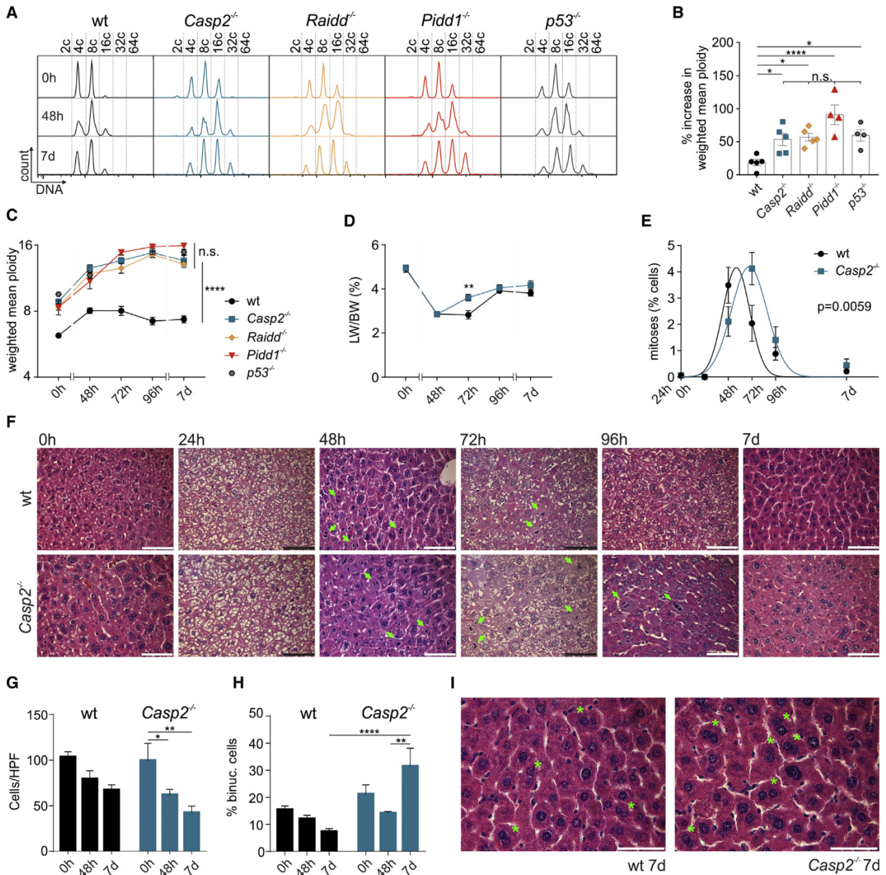
Figure 2. The PIDDosome Restricts Polyploidization during Liver Regeneration
