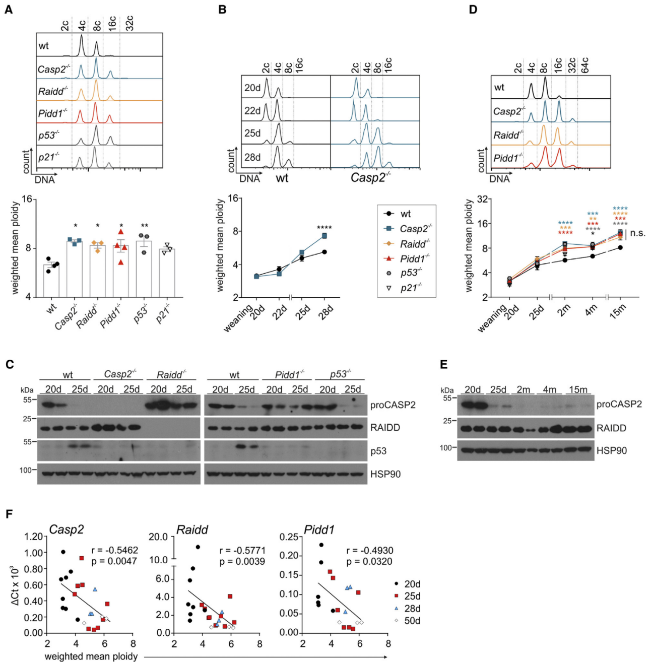
Figure 1. The PIDDosome-p53 Axis Regulates Hepatic Ploidy during Postnatal Liver Development
