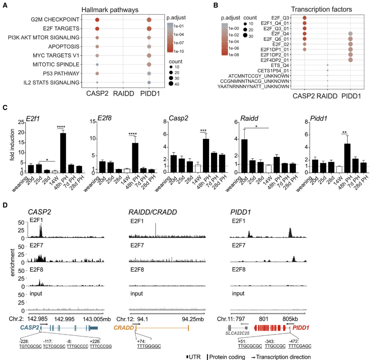
Figure 6. PIDD1 and CASP2 are Co-regulated with E2F Target Genes
