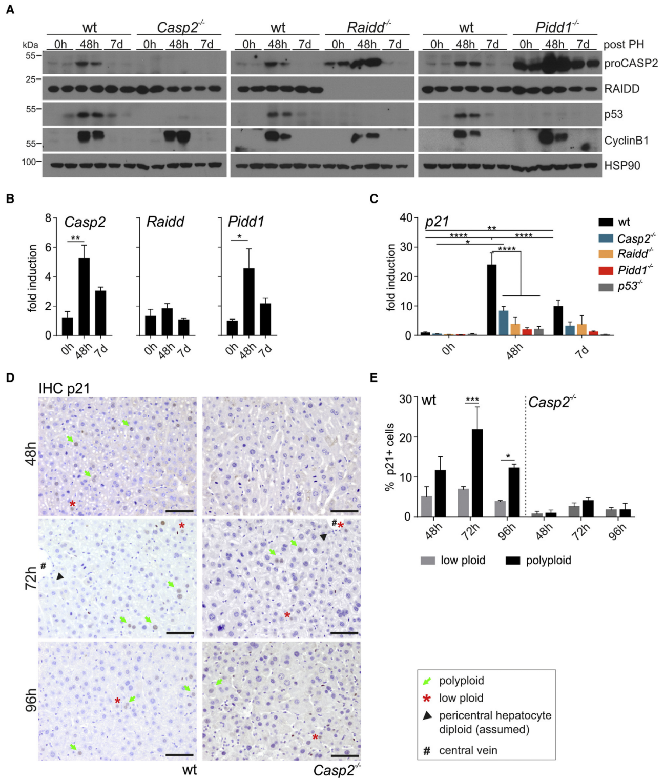
Figure 4. Adult Hepatocytes Induce and Activate the PIDDosome-p53-p21 Axis to Restrict Excessive Polyplodization during Regeneration (A) Immunoblot analysis assessing CASP2, RAIDD, p53, and cyclin B1 expression in hepatocytes isolated from 14-week-old mice (0 h) before and 48 h and 7 days after PH. (B) Transcript levels of Casp2 , Raidd , and Pidd1 in isolated hepatocytes also shown in (A).
