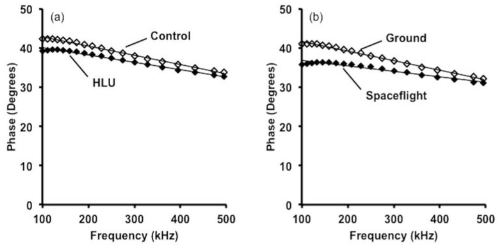
Figure 2. Plots of the average phase from a hind limb unloaded mouse and spaceflight mouse with controls. Dotted lines depict the method of calculating the 100-500 kHz phase-slope parameter.
