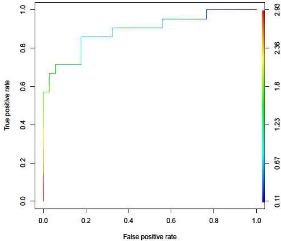
Fig 6. Receiver Operator Curve For Predicting Case Status
